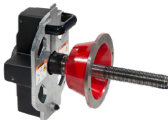
Ring protection for 22,5" alloy rim
